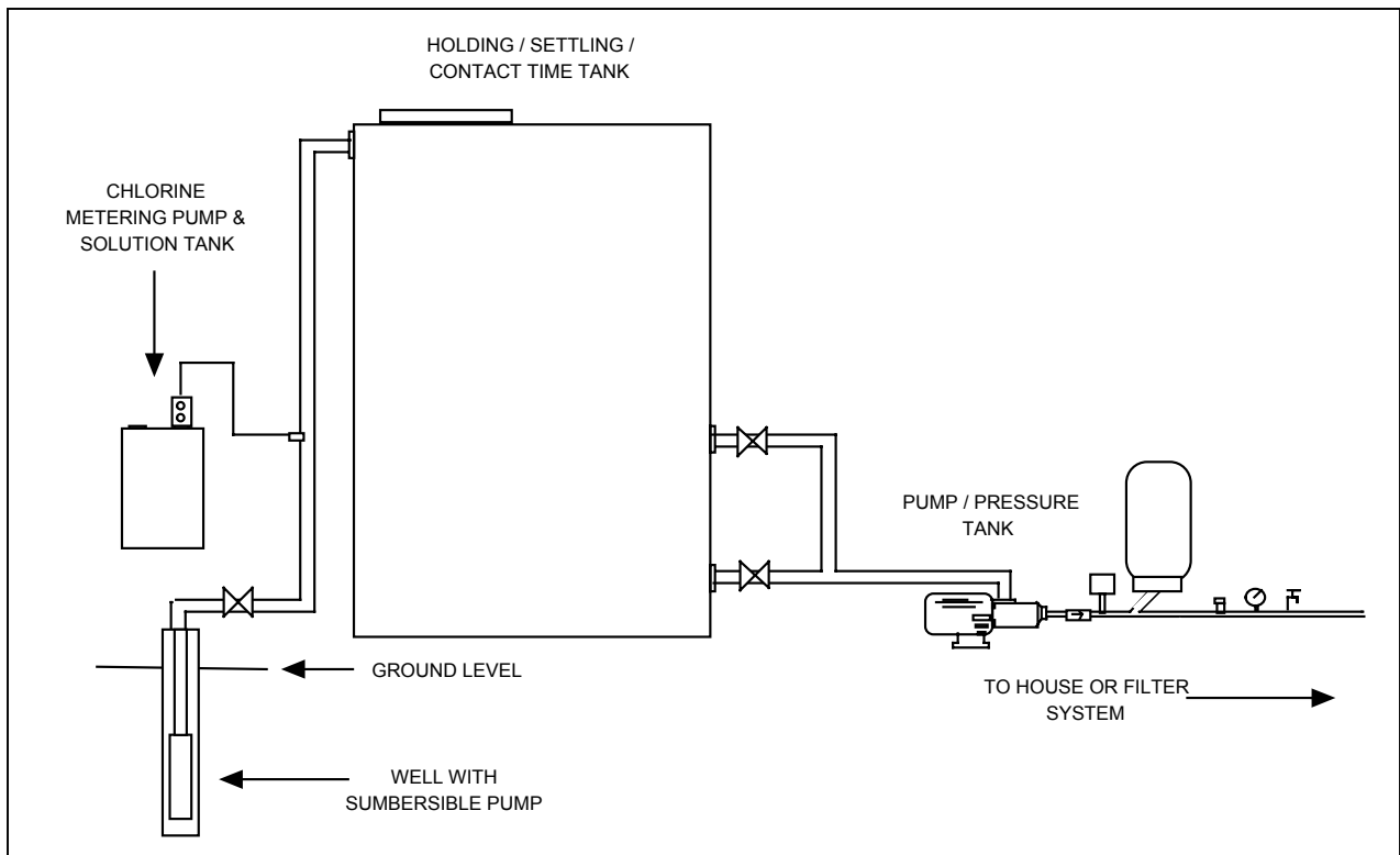
Figure 3 Chlorine Injection by Metering Pump & Holding/Contact Tank
