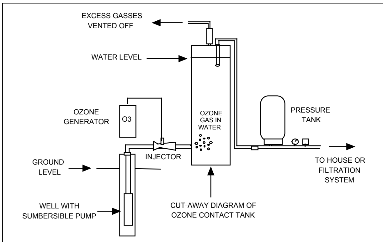
Figure 2 In-line Ozone Injection by Venturi & Contact Tank
