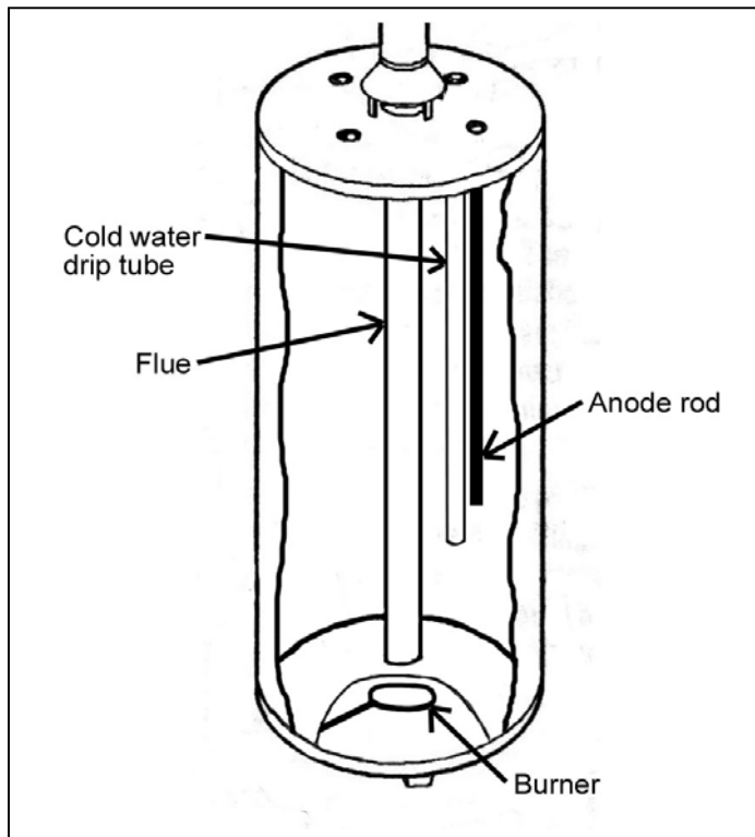
Figure 5 Typical gas water heater cut-away showing anode rod and cold water dip tube.
